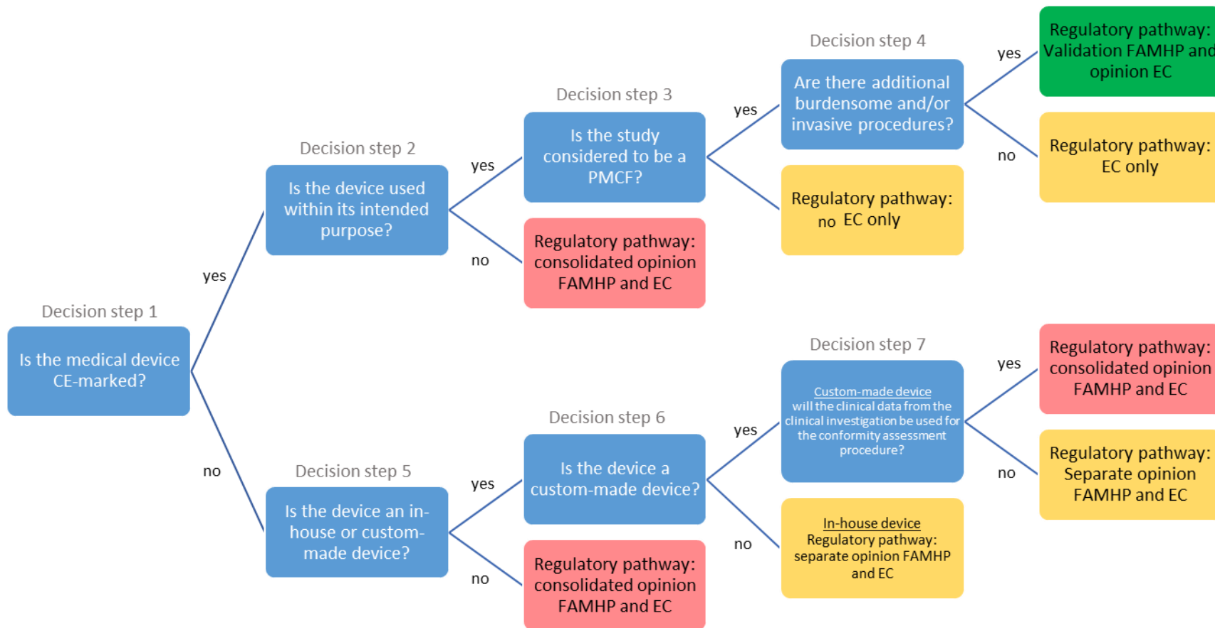
Figure 3. Decision tree
